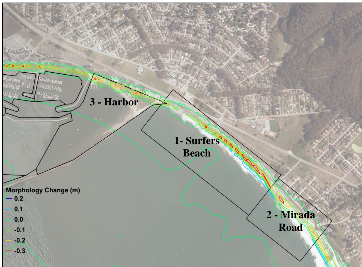
Figure 43. Erosion and accretion in vicinity of Surfer's Beach from June 2009 to November 2009 (6 months). The boxes (1 through 3) outline the analyses areas
