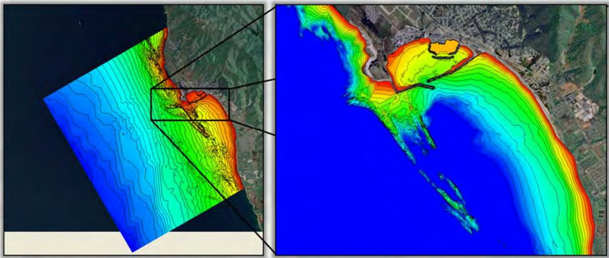
Figure 23. Composite bathymetry from all data sources
