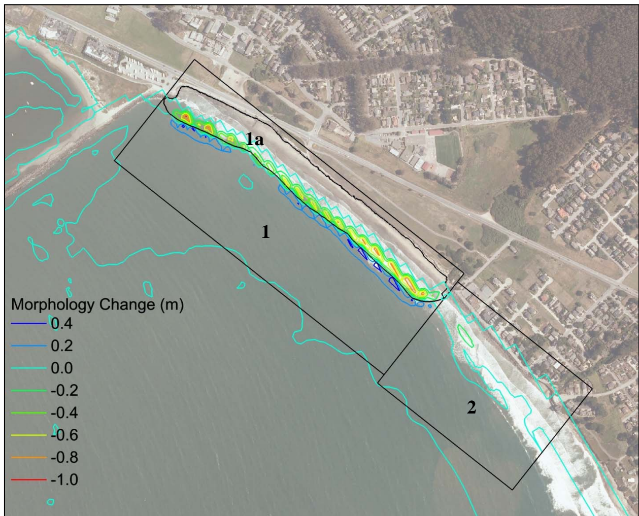
Figure 56. Erosion and accretion in vicinity of beach fill placement (240,000 yd 3 ) from June to November 2009. The boxes outline the analyses areas
